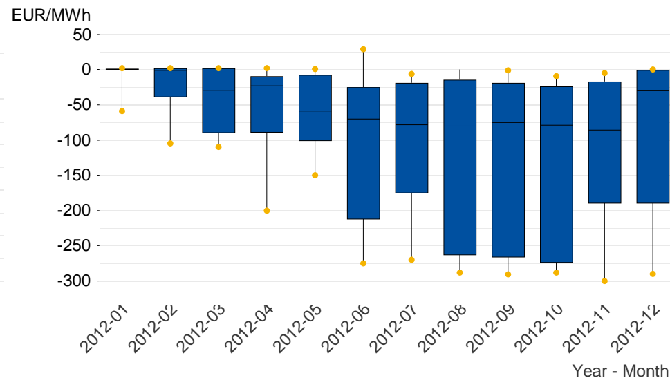
Secondary control energy in system sell direction
