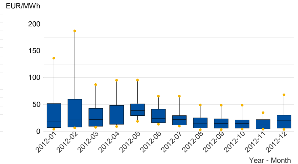
Secondary control capacity in system sell direction
