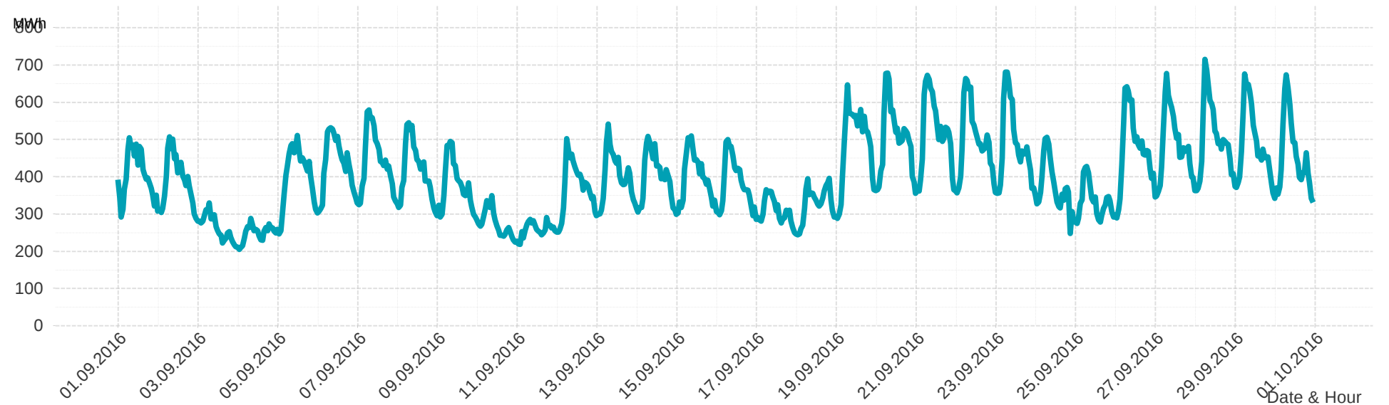
Consumption of the market area "Tirol & Vorarlberg" per hour
